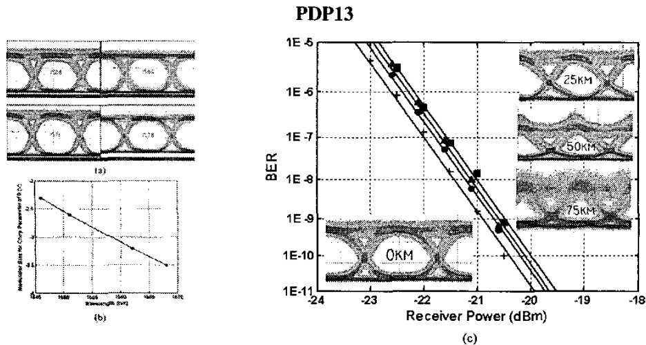
FIGURE 3. (a) Back-to-back eye diagrams from transmitter at wavelengths of 1558 nm, 1564 nm, 1571 nm, and 1578 nm. (b) Reverse bias zero chirp crossing point as a function of laser wavelength (c) BER curves and respective eye diagrams for back-to-back (cross), and transmission through 25 km (circles), 50 km (triangles), and 75 km (squares) of fiber at a wavelength of 1564 nm.
