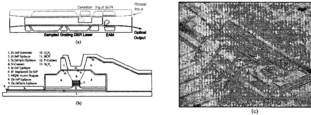
FIGURE 1. (a) Top view schematic of the device architecture, where the transmitter device used in this work is shown with a dark outline. (b) Cross-sectional schematic of modulator sections (c) Electron micrograph of completed transmitter device mounted on a carrier.
