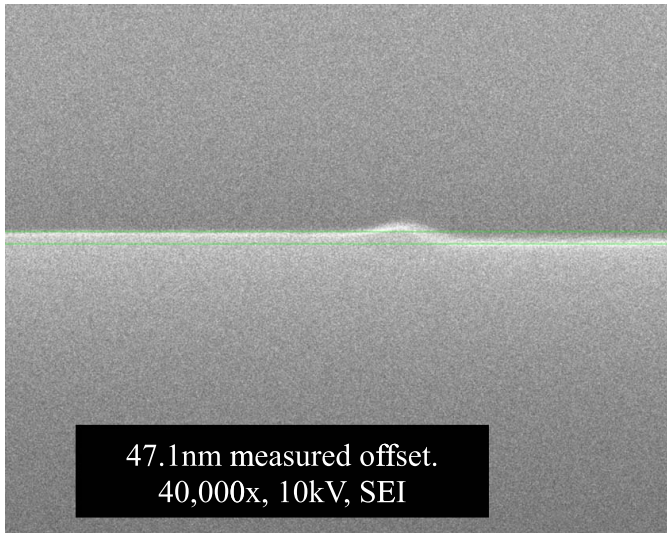
Fig. 3. An SEM image of the stitch on a 7 \mu m wide, 40nm thick waveguide. The green bars on the image specify the measured 47.1nm offset.
