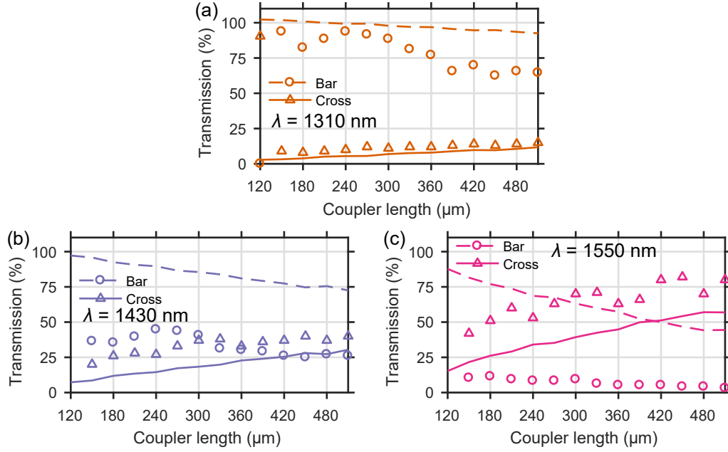
Figure 6.15: Transmission dependence on coupler length for (a) 1310 nm, (b) 1430 nm, and (c) 1550 nm wavelengths input including overlaid simulations for each.
