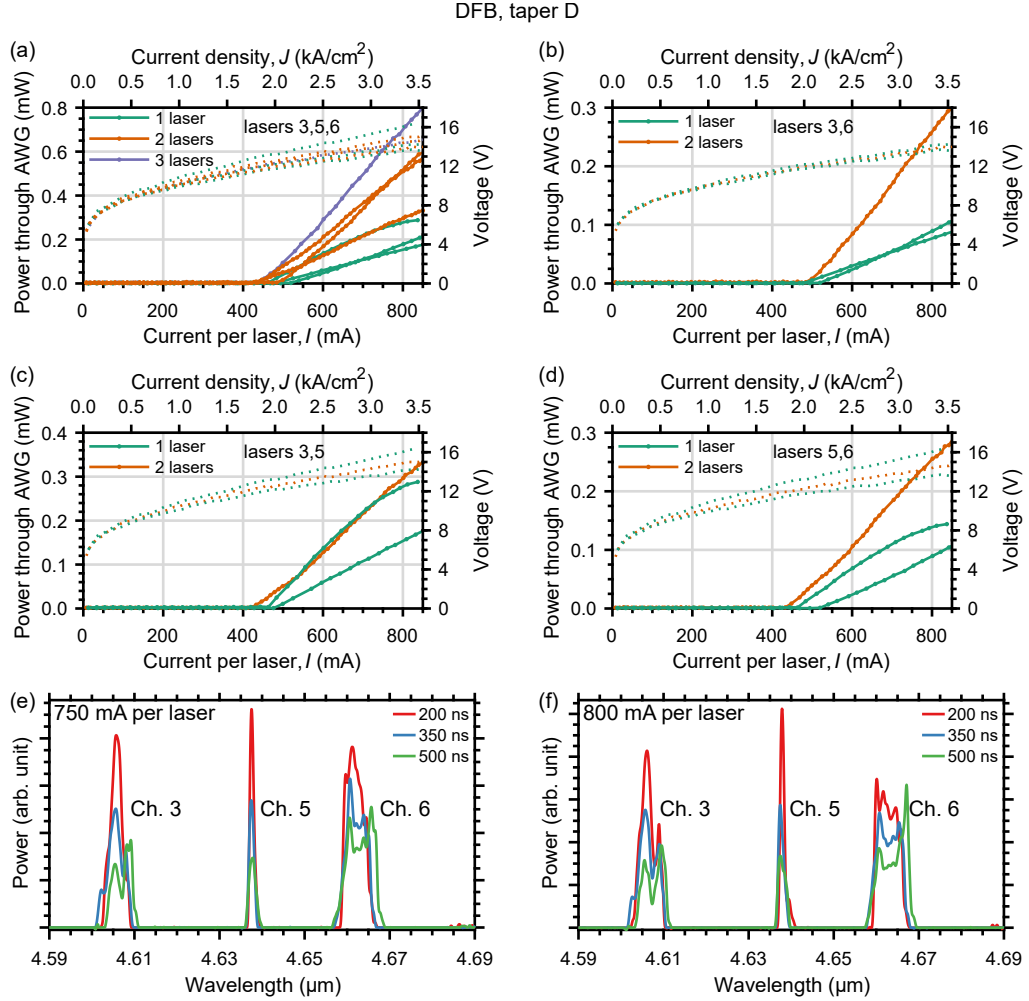
Figure 7.20: LIV plots of a multi-spectral three-channel DFB while driving laser channels (a) 3, 5, and 6; (b) 3 and 6; (c) 3 and 5; (d) 5 and 6. Spectra of the simultaneously driven three-channel DFB laser for three different pulse widths with (e) 750 mA and (f) 800 mA drive current per laser.
