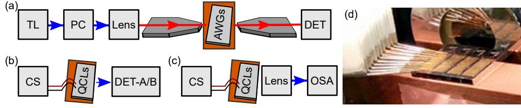
Figure 7.9: Experimental setups for (a) AWG passive transmission, (b) QCL LIV, and (c) QCL spectral measurements. (d) A photograph of the QCL LIV setup with DET-A is shown.
