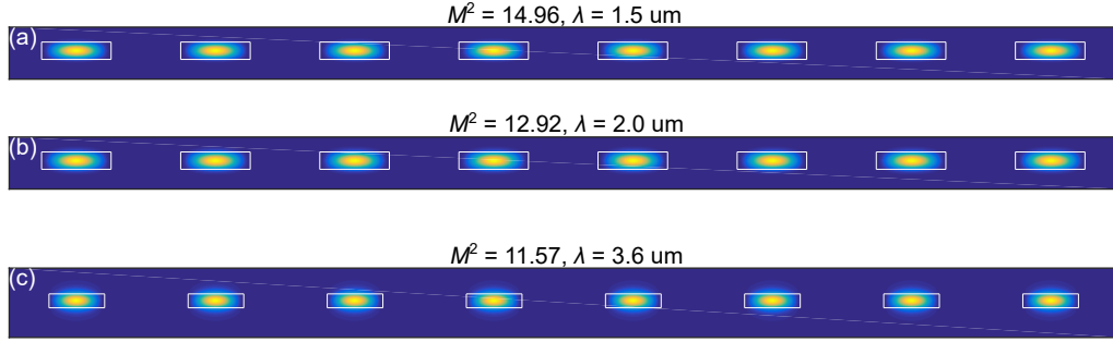
Figure 3.10: Beam quality comparison of arrays of SOI outputs with 0.5- \mu\text{m} thickness and 2.0- \mu\text{m} width for (a) 1.5 \mu\text{m} , (b) 2.0 \mu\text{m} , and (c) 3.6 \mu\text{m} wavelengths.
