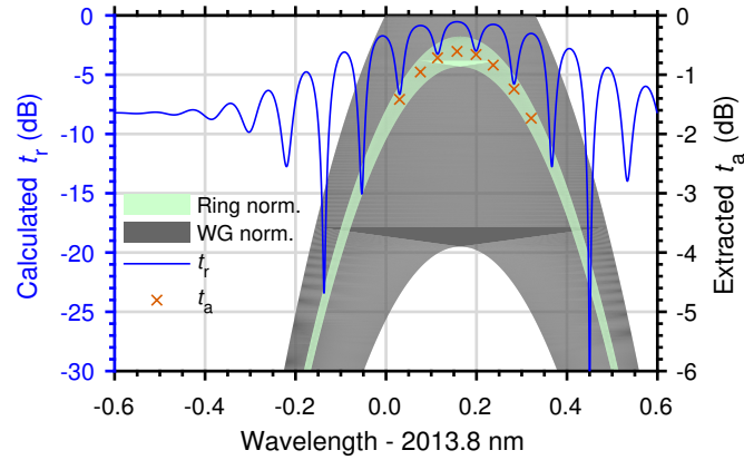
Figure 4.23: Uncertainty comparison between the waveguide normalization method and the AWG-ring method.
