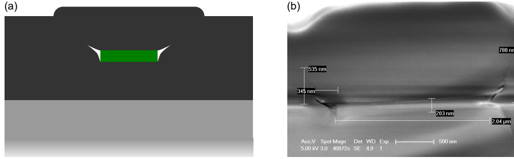
Figure 6.17: (a) Schematic and (b) SEM of air-gap “bunny ear” formation from sputtered \text{SiO}_2 at the corners of the waveguide.
