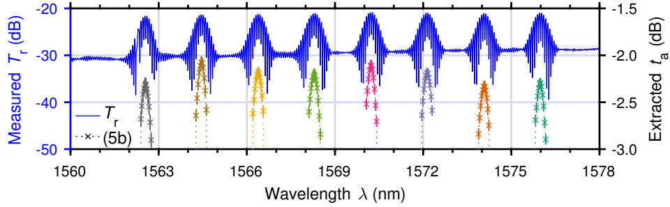
Figure 4.17: (Left axis) Measured AWG-ring off-chip transmission spectrum T_r and (right axis) on-chip transmission spectra t_a extracted for each AWG channel using (4.12b).
