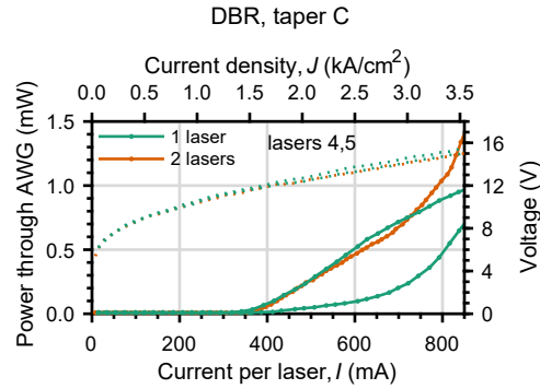
Figure 7.23: LIV plots of a multi-spectral two-channel DBR with taper design C while driving laser channels 4 and 5.
