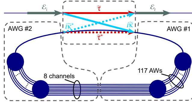
Figure 4.7: Diagram of the AWG-ring with complex amplitudes \mathcal{E}_i and \mathcal{E}_t of the input and output guided electric fields. Coupling between the bus and ring waveguides is characterized by \tilde{\tau} and \tilde{\kappa} .
