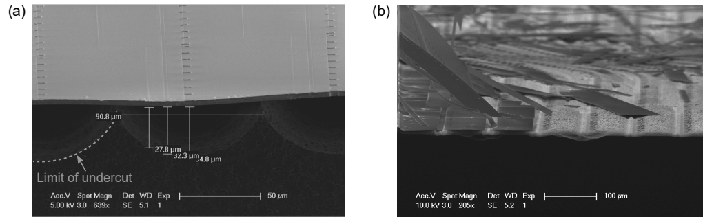
Figure 6.18: SEMs of the \text{XeF}_2 undercut of the Si substrate: (a) successful undercut and (b) failure do to excessive undercut at the facets.
